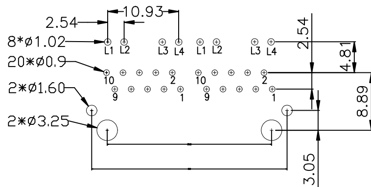
SUGGESTED PCB PAD LAYOUT COMPONENT SIDE VIEW
