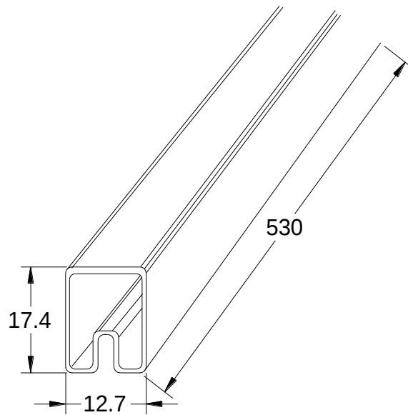
Tube: 530*12.7*17.4mm
