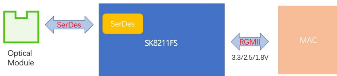
Figure 4. Fiber (FIBER<->RGMII) Application
