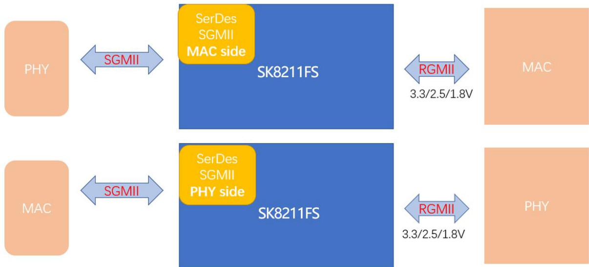
Figure 6. SGMII to RGMII Application
